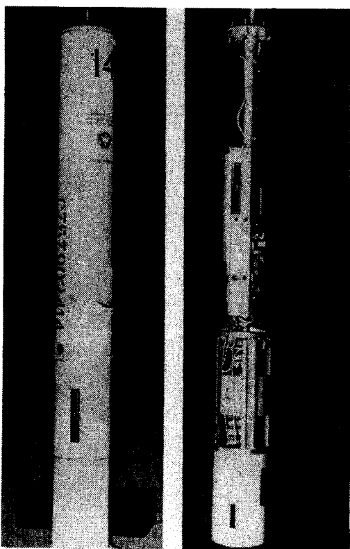
SOVIET "75" SONOBUOY
